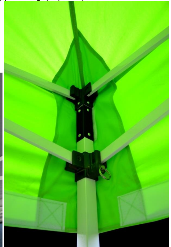
5. Corner velcros / double layer material reinforcement/ CFRP joints
